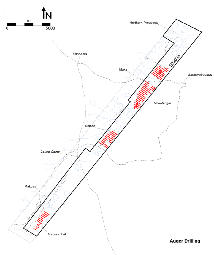
Figure 7: Auger Drilling Coverage Map
