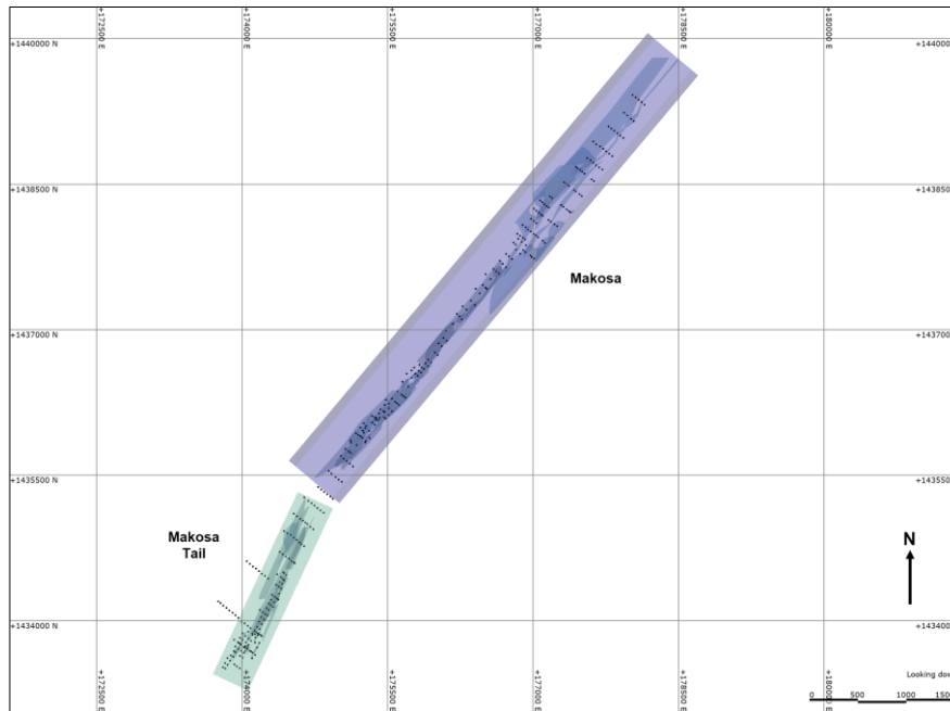
Figure 28: Plan View Showing Arrangement of Block Models
