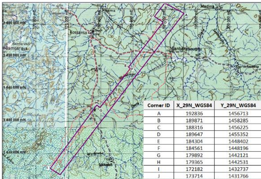
Figure 2: E02038 Licence Location and Definition
