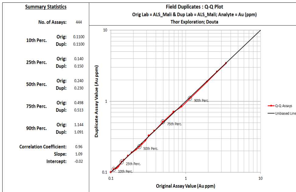
Figure 17: Field Duplicate Q-Q Plot
