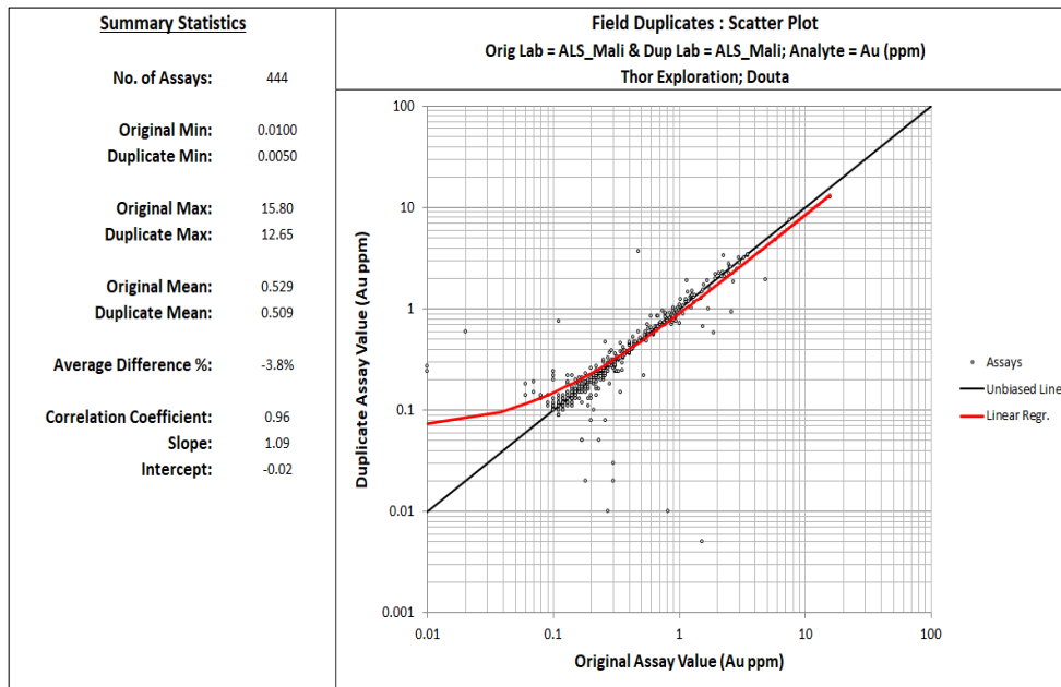
Figure 16: Field Duplicate Scatter Plot
