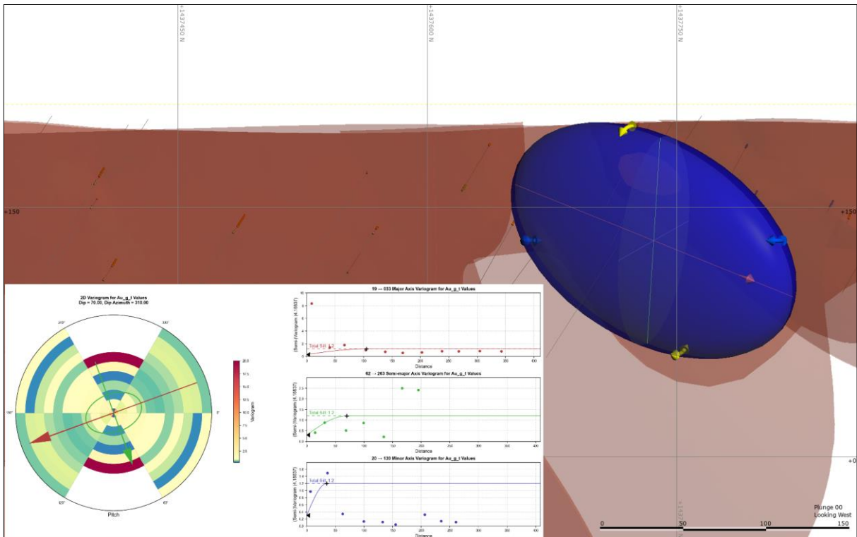
Figure 25: Longitudinal Visual Representation of Makosa Variogram
