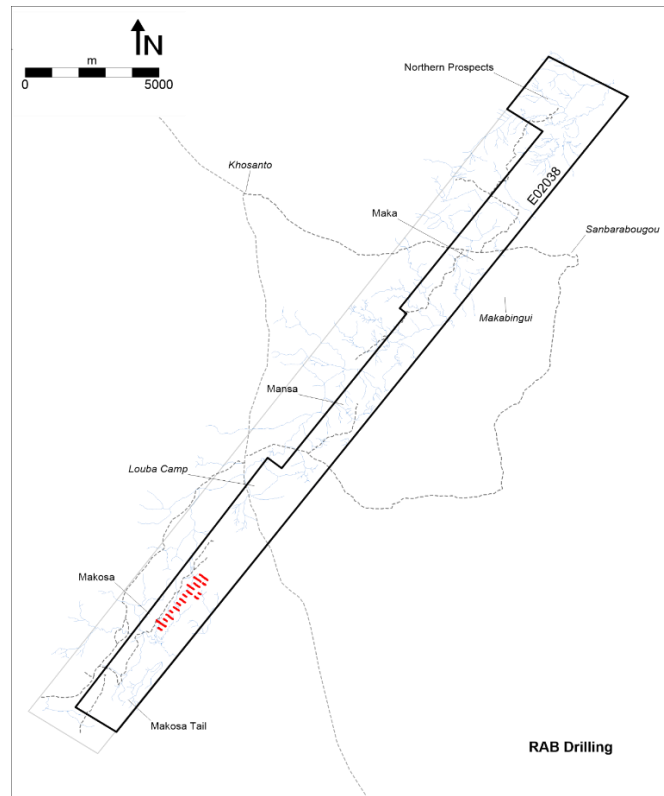
Figure 10: RAB Drilling Coverage Map
