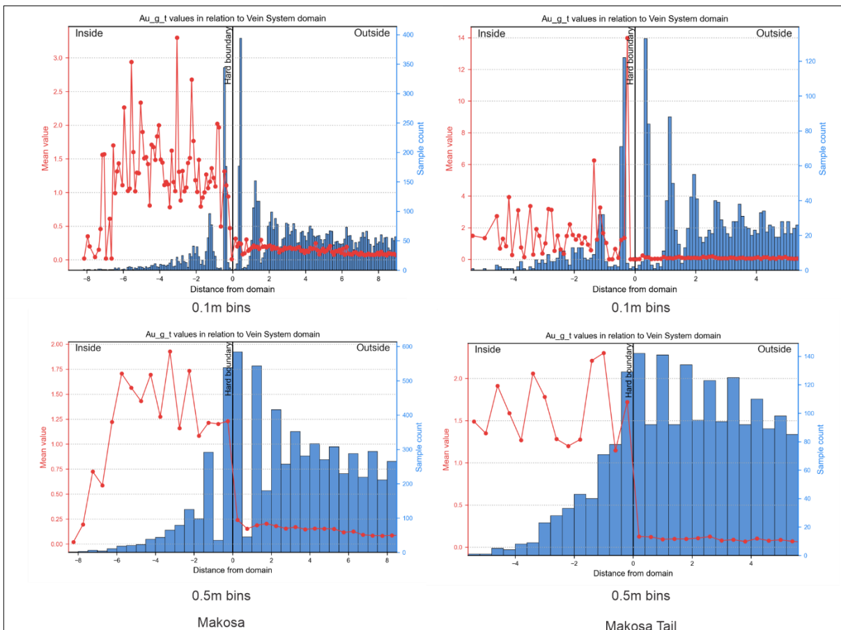
Figure 23: Domain Boundary Validation Plots
