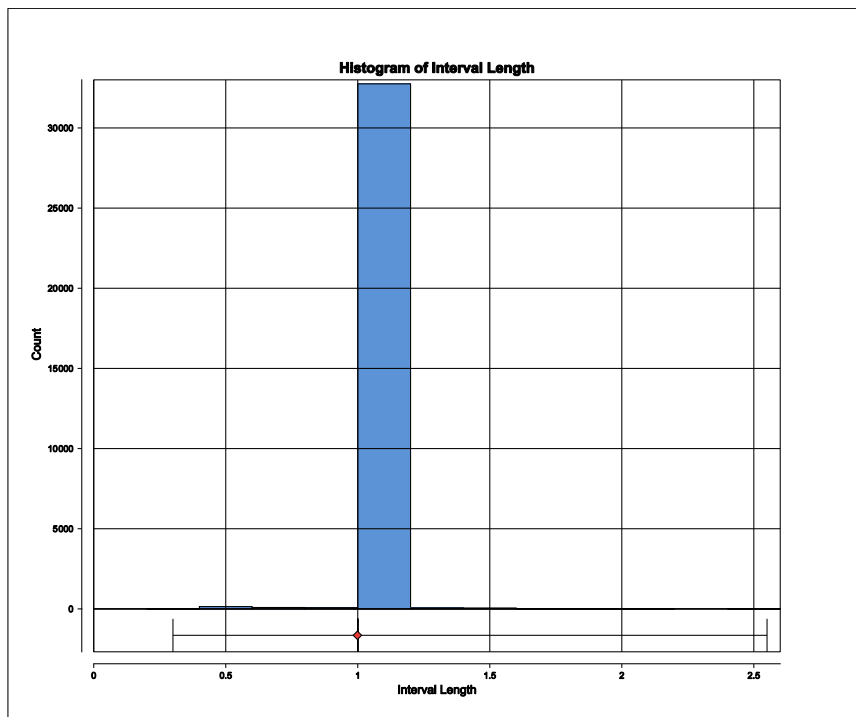
Figure 22: Histogram of Total Population Interval Length
