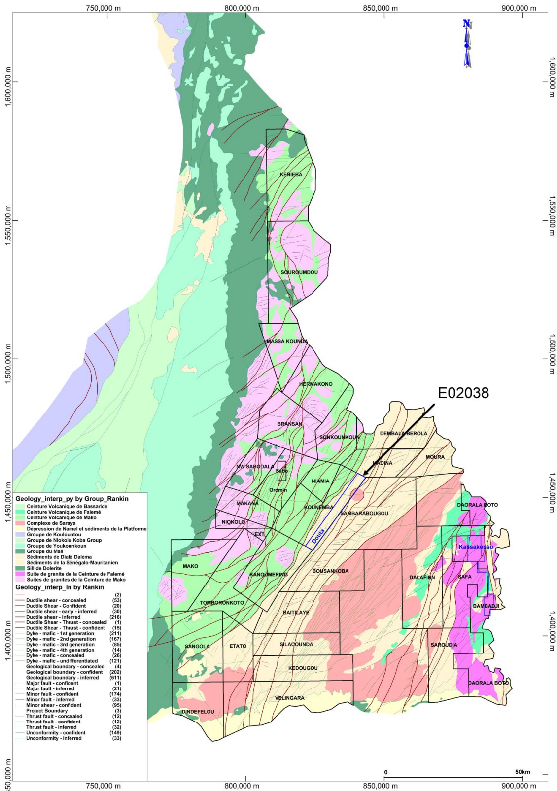
Figure 5: Regional Geological Setting of the Douta Licence
