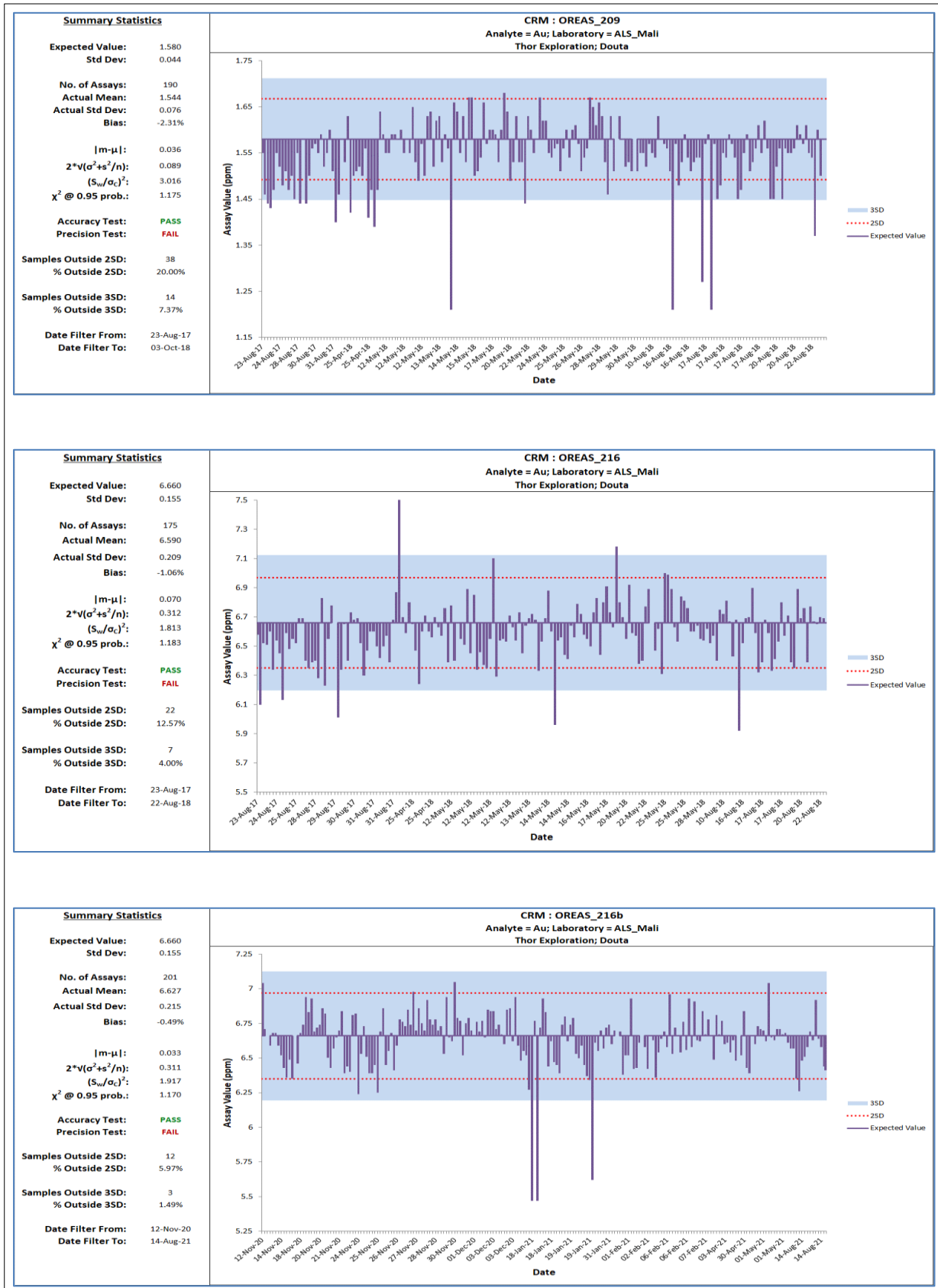
Figure 18: CRM Performance Charts: OREAS_209 (top), OREAS_216, OREAS_216b
