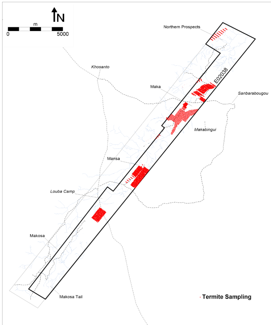
Figure 8: Termite Mound Sample Coverage Map
