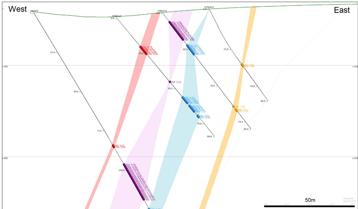
Figure 20: Cross section through Makosa showing conformable mineral domains
