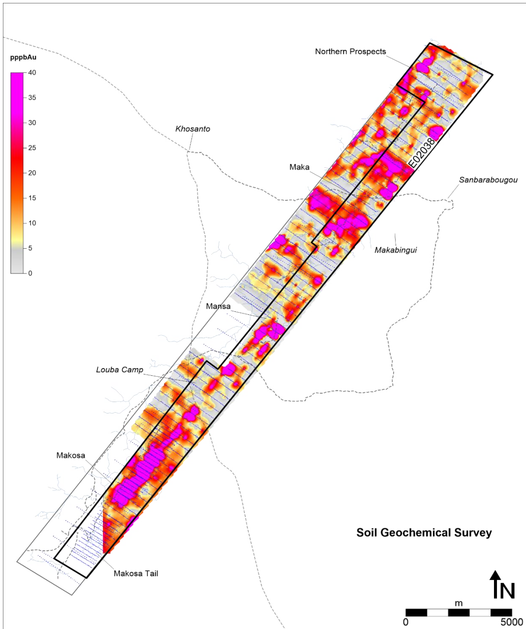
Figure 3: Soil Geochemical Survey Coverage Map
