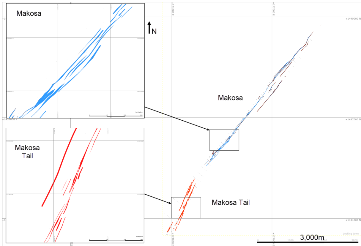
Figure 21: Plan View showing orientations of Makosa and Makosa Tail
