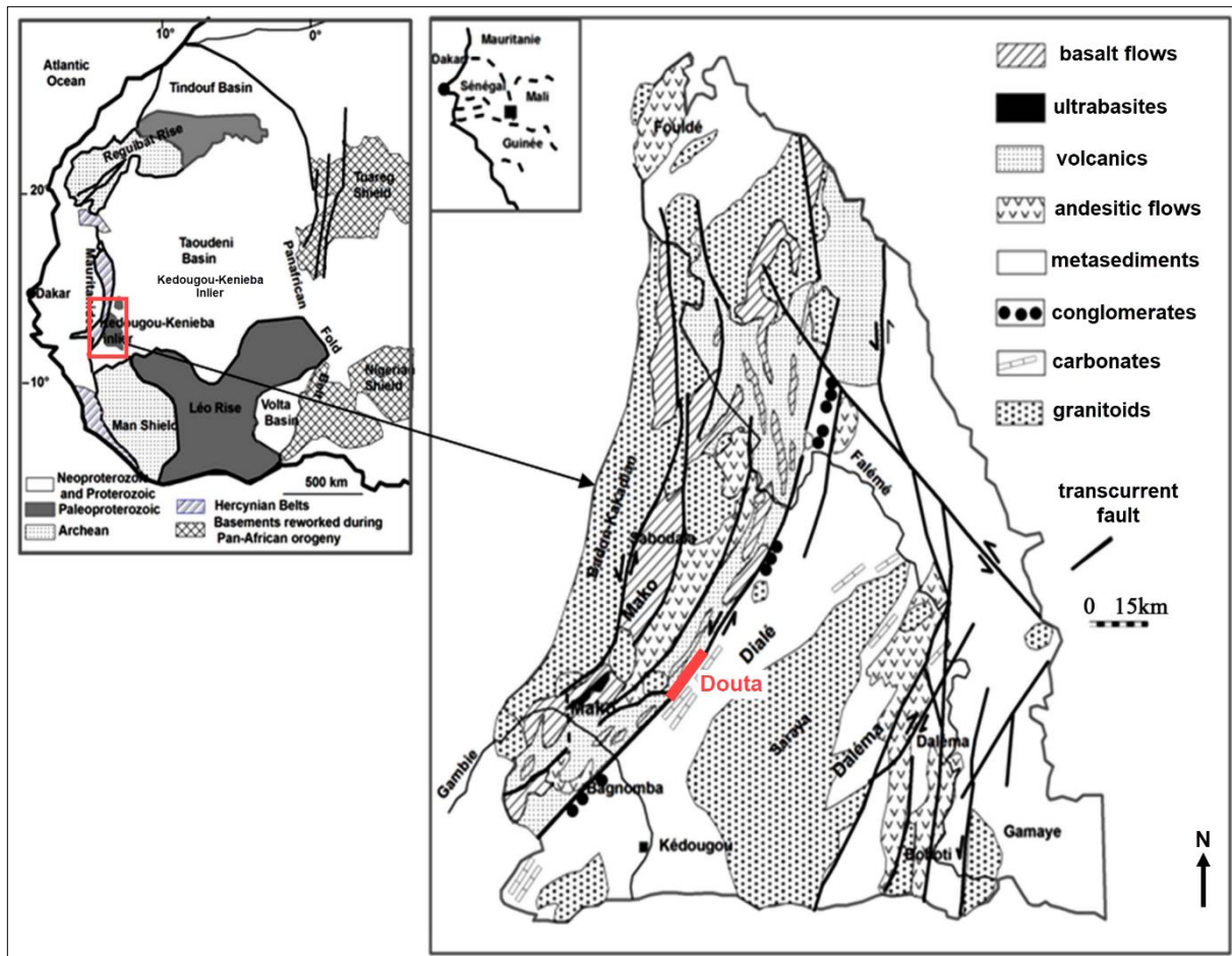
Figure 4: Geology of West Africa and Kendougou-Kenieba Inlier (after Diene, et al,2012)
