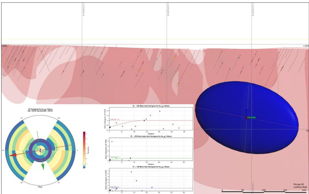
Figure 26: Longitudinal Visual Representation of Makosa Tail Variogram
