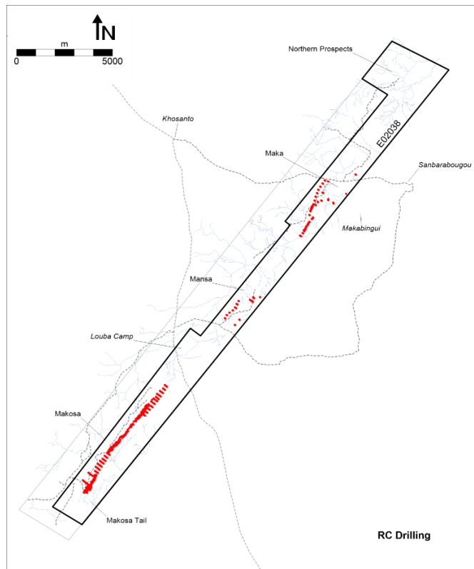
Figure 11: RC Drilling Coverage Map
