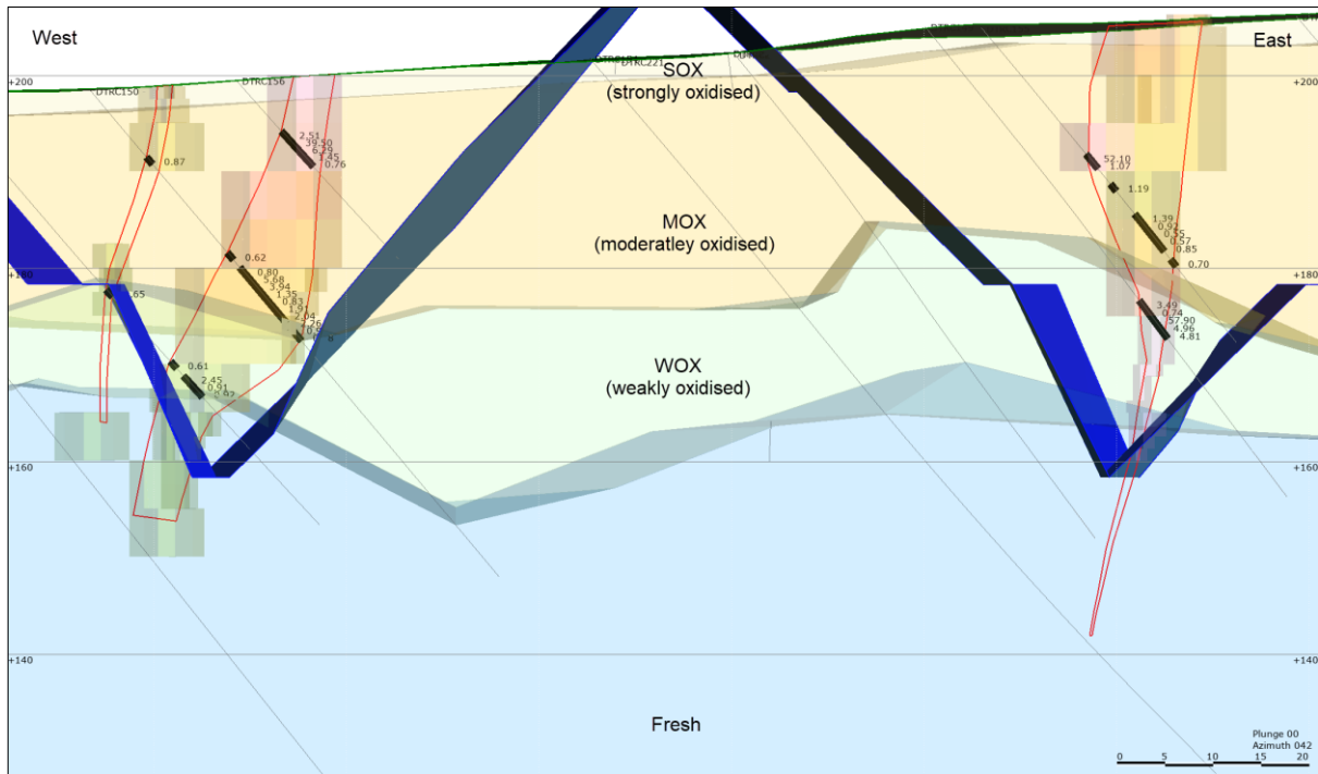
Figure 27: Cross Section through Makosa Tail Showing Weathering Profile
