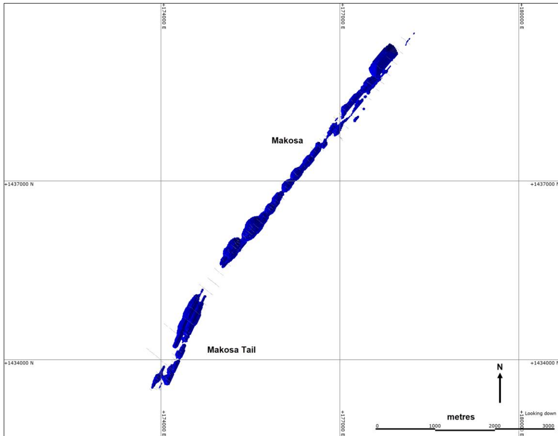
Figure 33: Plan View Showing Makosa and Makosa Tail Pit Shells
