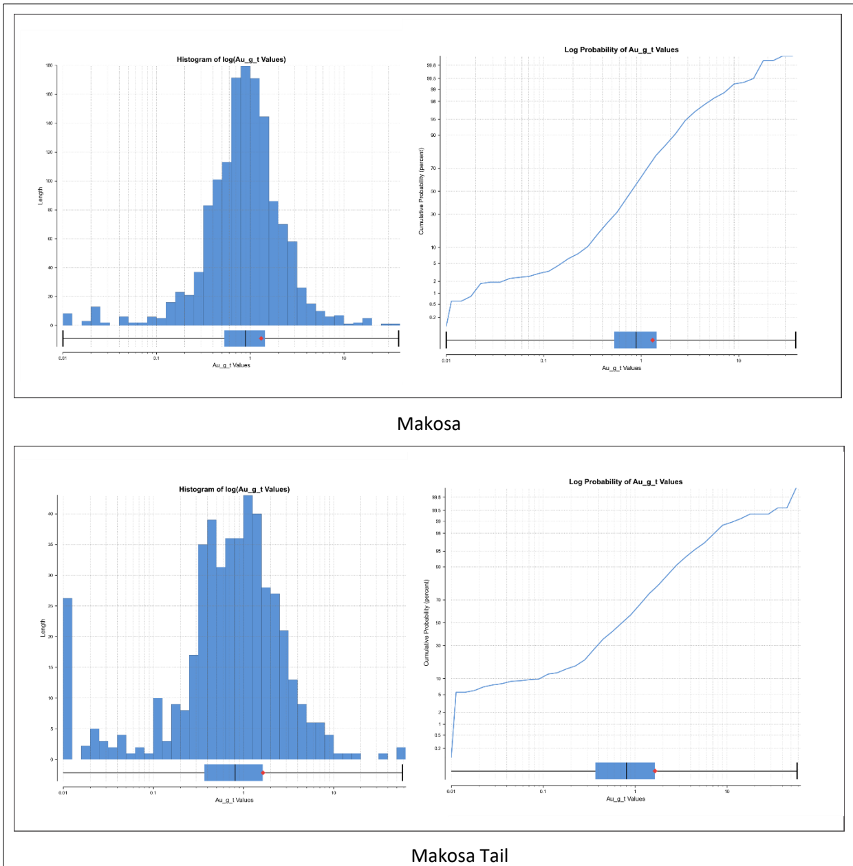
Figure 24: Log Histograms and Log Probability Plots for Composited Intervals
