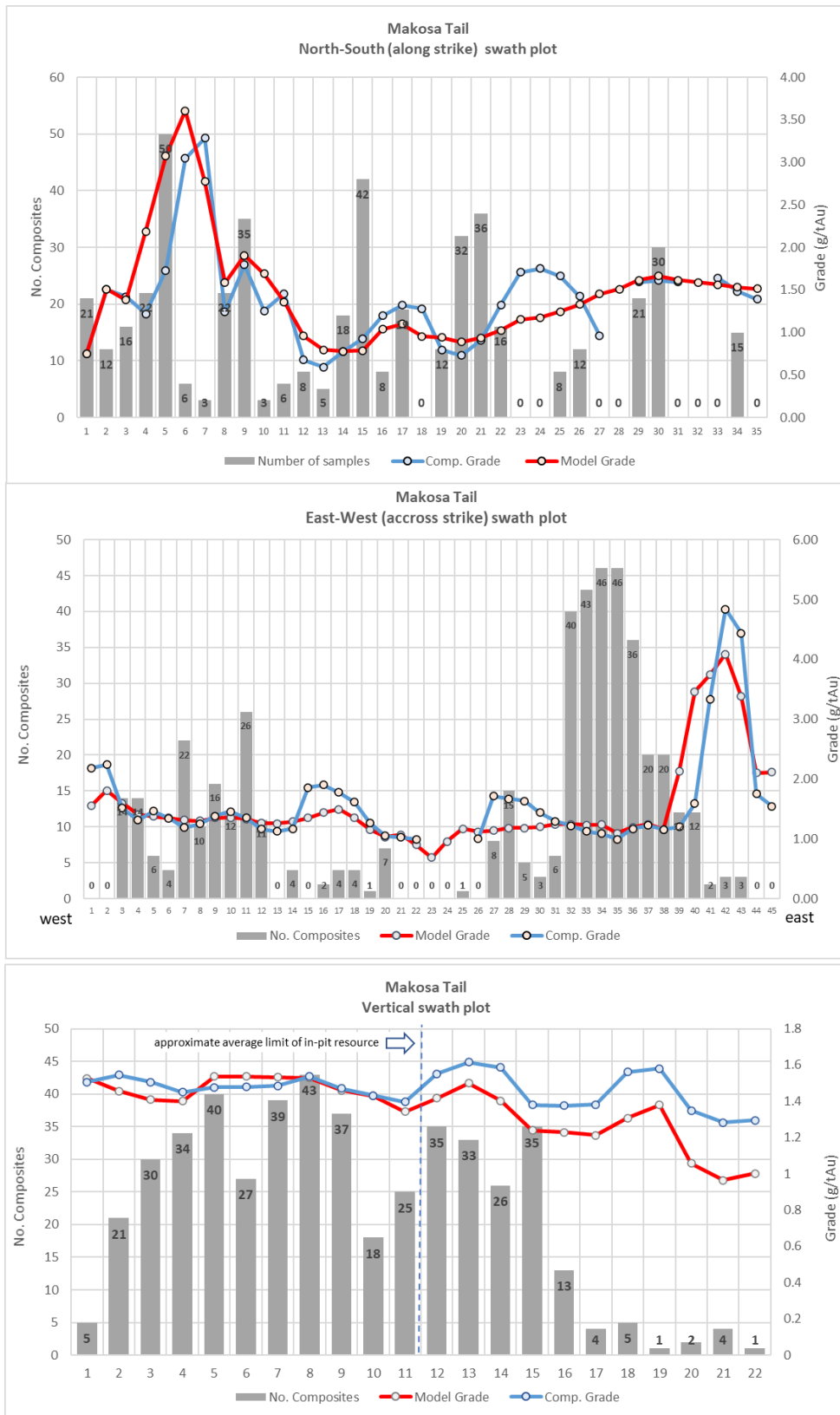
Figure 30: Makosa Tail Swath Plots
