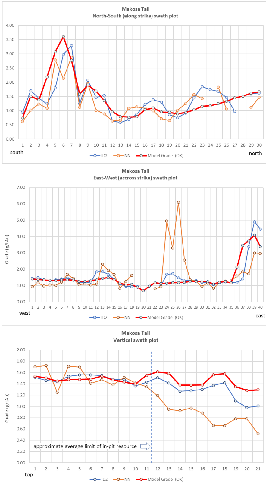
Figure 32: Comparisons between Different Estimation Techniques - Makosa Tail
