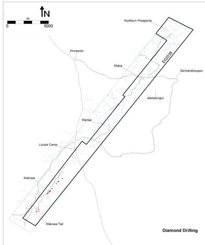
Figure 12: Diamond Drilling Coverage Map
